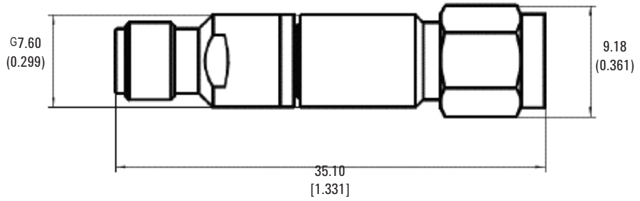
Figure 3. N9398/99C product outline
