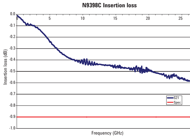
Figure 7. N9398C typical insertion loss versus frequency
