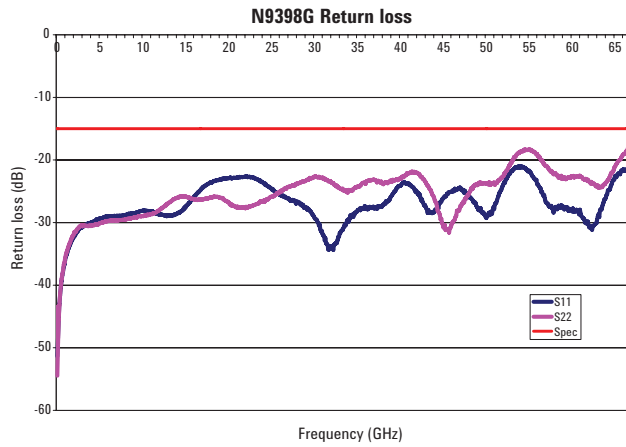
Figure 14. N9398G typical return loss versus frequency
