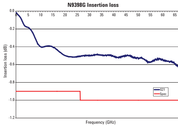
Figure 15. N9398G typical insertion loss versus frequency
