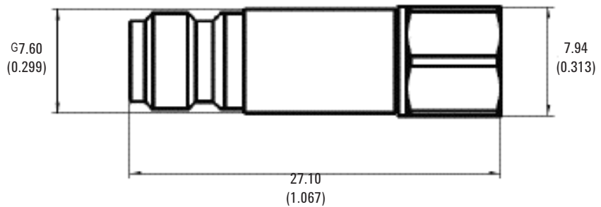
Figure 5. N9398G product outline
