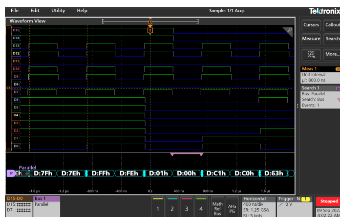
Digital channel trigger and decode
