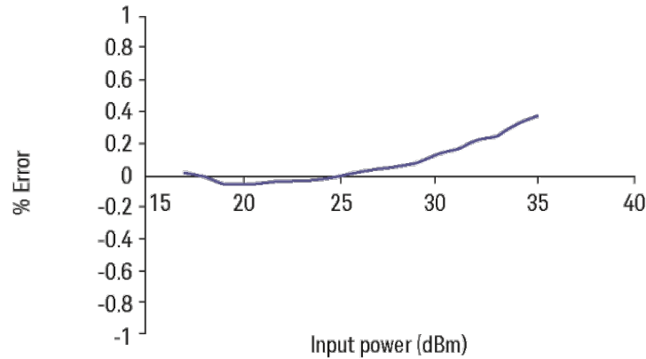
Typical N8481H/2H power linearity at 25°C, after zero and calibration with associated measurement uncertainty
