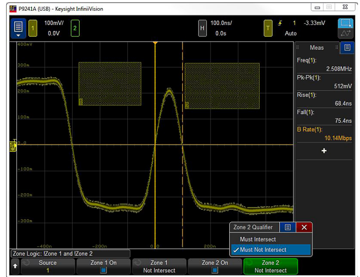
Zone Trigger enable quick and easy isolation of the data pattern of interest.
