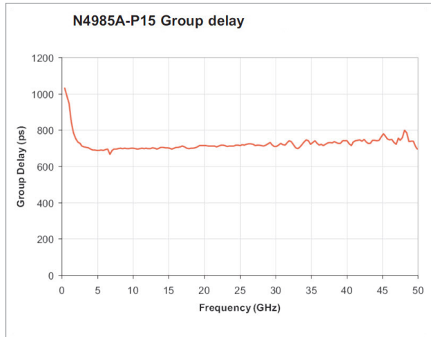
Figure 2. Group delay
